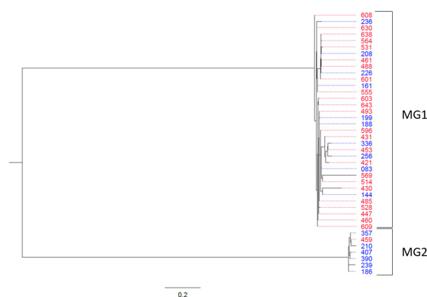
Figure 2 Phylogenetic tree of Mycoplasma genitalium -positive samples using dual locus sequence typing. Red denotes samples collected pre-MDA and blue denotes samples collected post-MDA; bootstrap value between MG1 and MG2=100%. Scale: mean number of nucleotide substitutions per site. MDA, mass drug administration.
